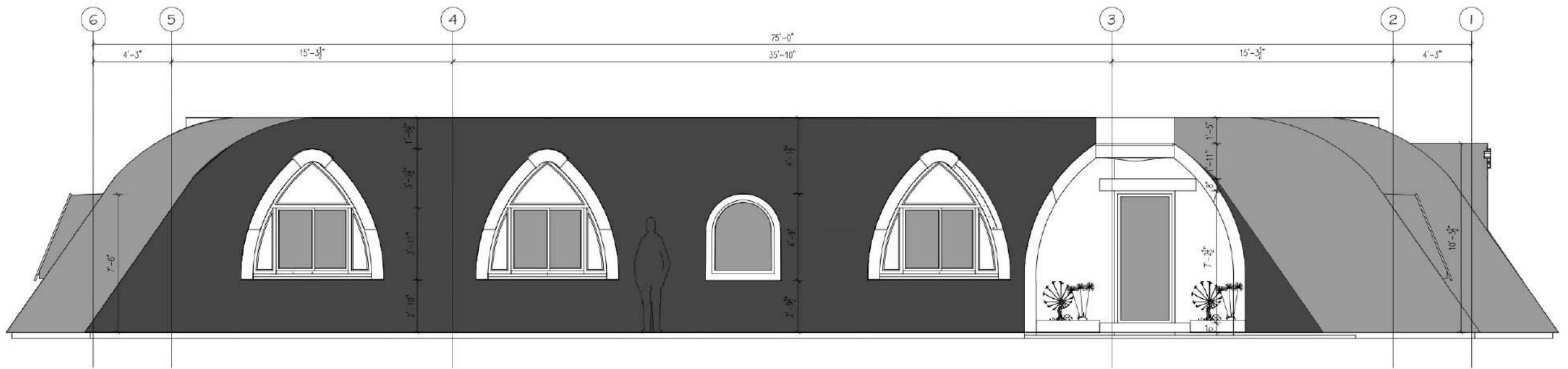
SCALE = 1/4" : 1'-0" 2 A5 REAR ELEVATION
