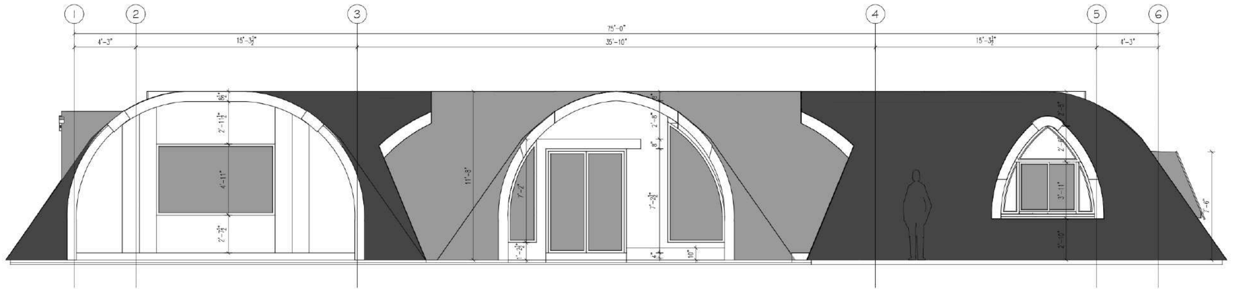
SCALE = 1/4" : 1'-0" 1 A5 FRONT ELEVATION
