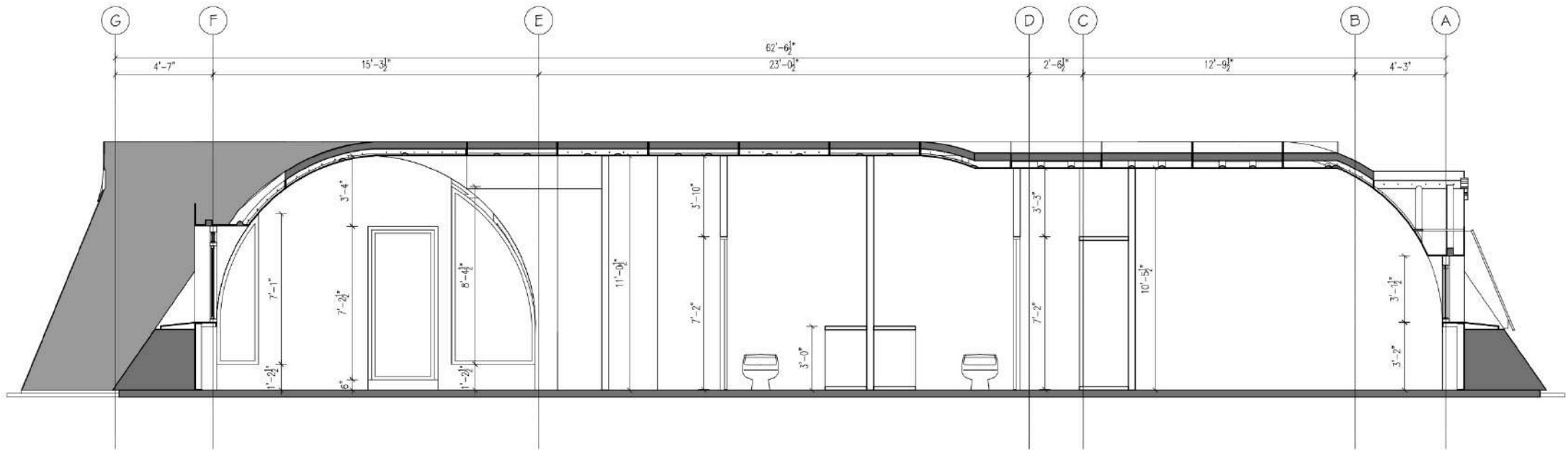
SCALE = 1/4" : 1'-0" 2 A5 BUILDING SECTION - 2
