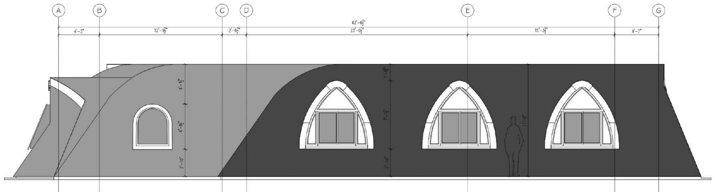
SCALE = 1/4" : 1'-0" 4 A5 LEFT ELEVATION
