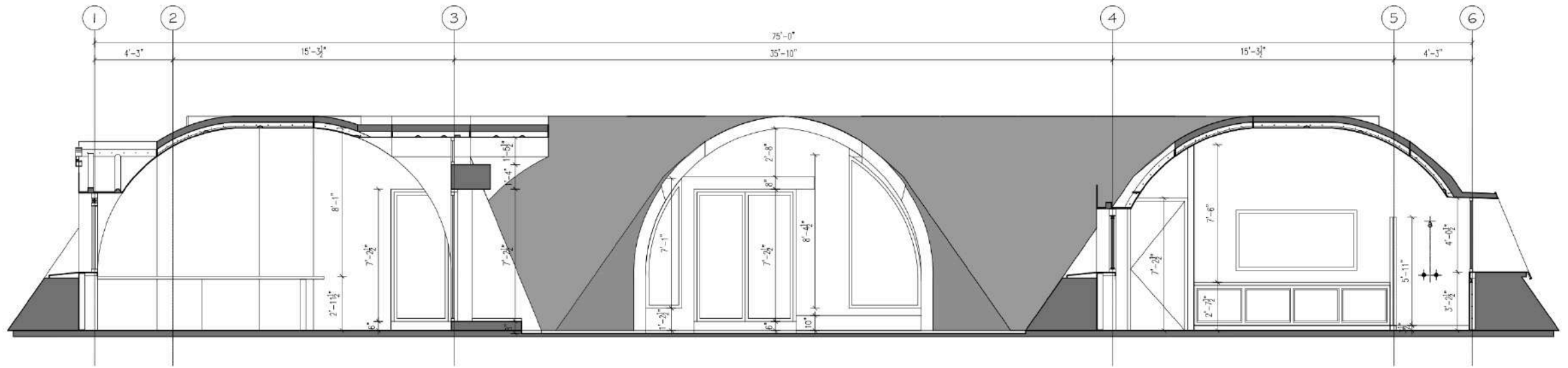
SCALE = 1/4" : 1'-0" 1 A5 BUILDING SECTION - 1
