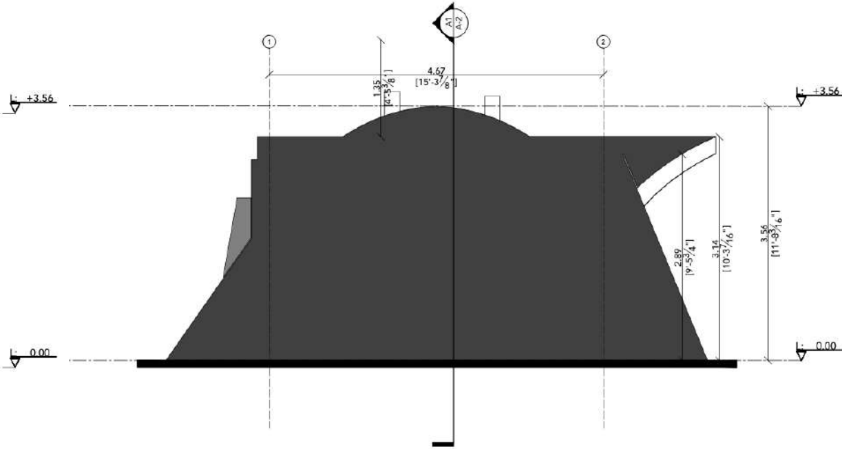
SCALE = 1:50 2 A2 ELEVATION 2
